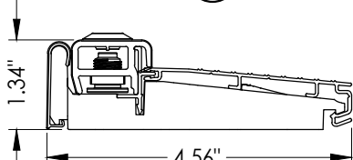
17 INSWING ADJUSTABLE THRESHOLD ZAI4565RDS
