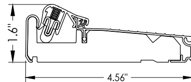
21 INSWING ARTICULATING THRESHOLD ZACAA4565FN
