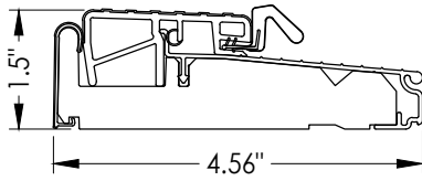
24 OUTSWING THRESHOLD ZOB4565FN
