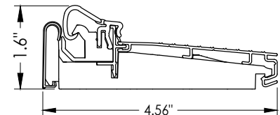
22 INSWING ARTICULATING THRESHOLD ZAC4565RDS
