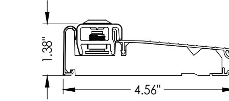
14 INSWING ADJUSTABLE THRESHOLD ZAI4565FN
