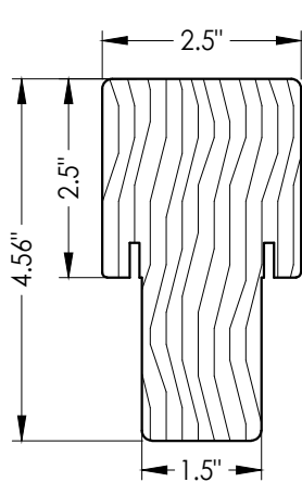
2 INTEGRAL MULLION
