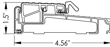
23 OUTSWING THRESHOLD ZOBL4565
