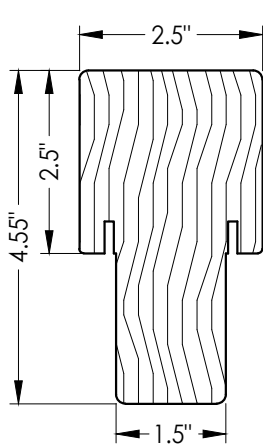
2A INTEGRAL MULLION FrameSaver (Endura)
