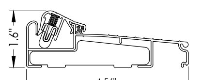
20 INSWING ARTICULATING THRESHOLD ZACLAA4565
