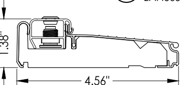
16 INSWING ADJUSTABLE THRESHOLD ZAI4565FN
