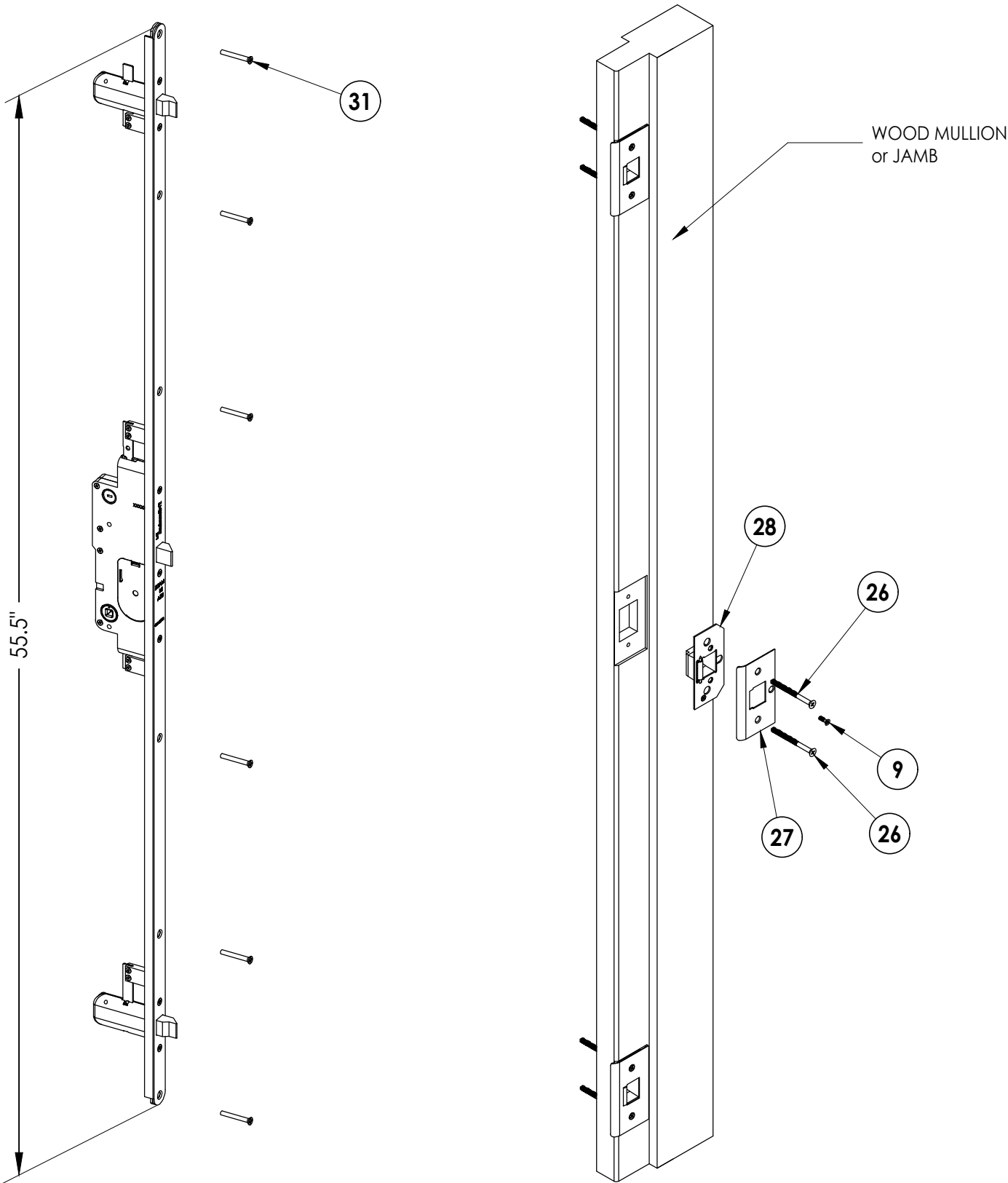
Trilennium® 3000 3 Point Lock
