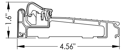
18 INSWING ARTICULATING THRESHOLD ZACL4565
