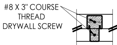
DETAIL 1
