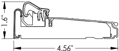
19 INSWING ARTICULATING THRESHOLD ZAC4565FN
